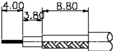
Cable preparation
