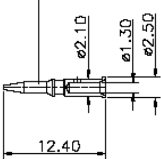
Central Contact
